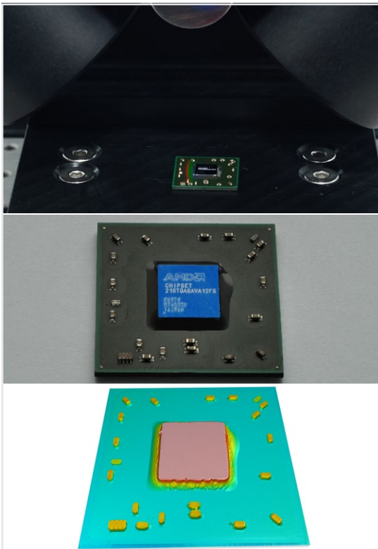
Dimension inspection after packaging
